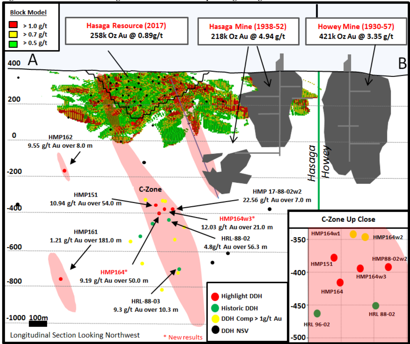
Figure 2 Schematic Longitudinal Section of Deep Hasaga Targets
